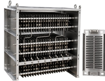
Punched Grid Resistors, Solenoids & AC Brakes
