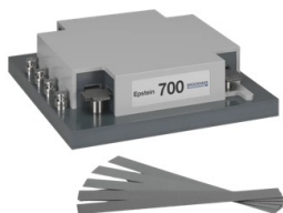
Epstein Apparatus (Core Loss Analysis)
